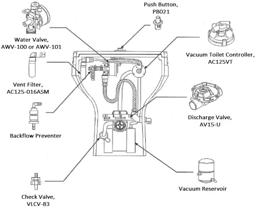
AIRVAC Vacuum Toilet Diagram
